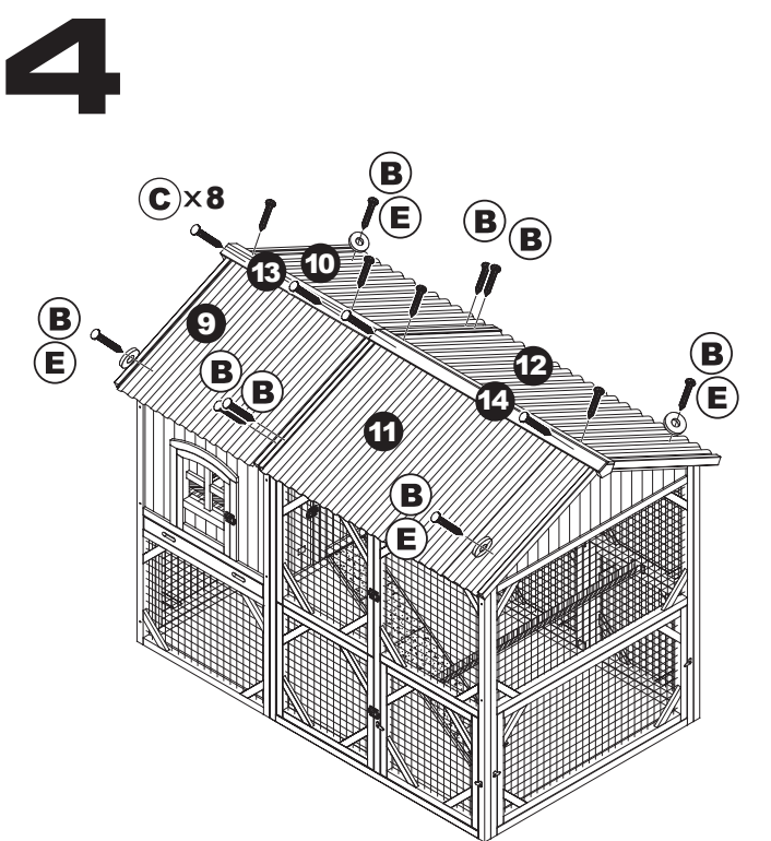
Attach Roosting Area Roof (9, 10) and Foraging Area Roof (11, 12) with Screws (B) and Plastic Washers (E). Attach Roosting Area Roof Cap (13) and Foraging Area Roof Cap (14) with Screws (C).
