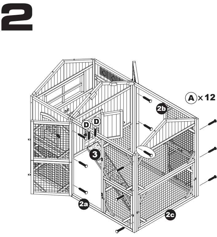
Connect Foraging Area Panels (2a, 2b, 2c) to Roosting Area with Screws (A). Attach Ramp (3) with Screws (D).
