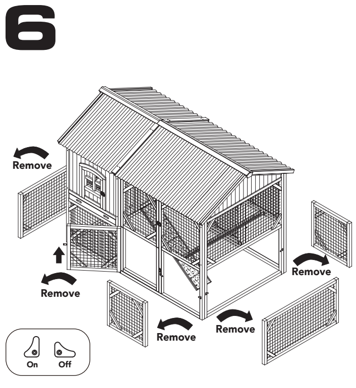
Bottom panels can be removed by turning the lock.
