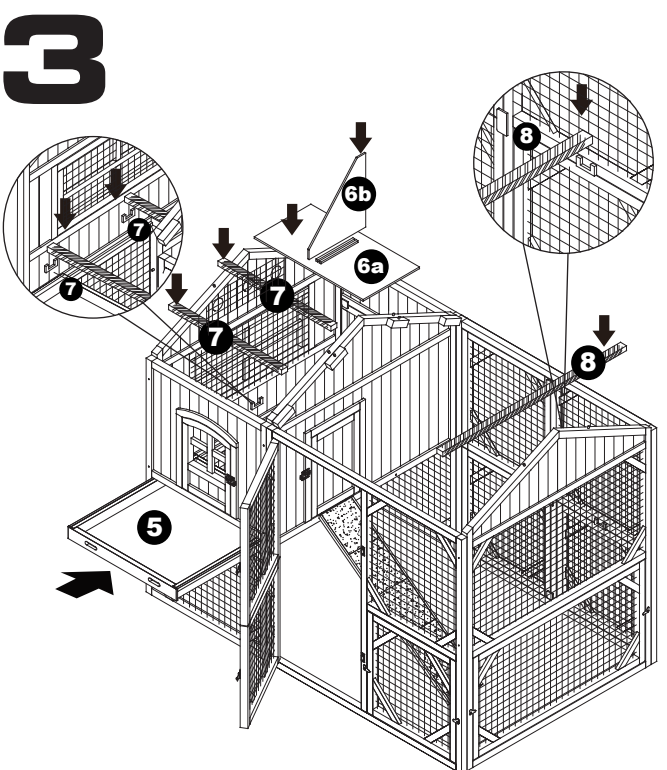
Insert Cleaning Tray (5). Insert Nesting Box Board (6a). Insert Nesting Box Divider (6b). Insert Internal Roosting Bars (7). Insert External Roosting Bar (8).
