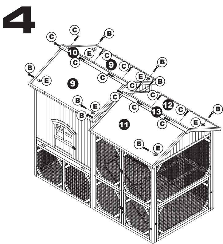
Attach Roosting Area Roof (9) and Foraging Area Roof (11, 12) with Screws (B) and Plastic Washers (E). Attach Roosting Area Roof Cap (10) and Foraging Area Roof Cap (13) with Screws (C).
