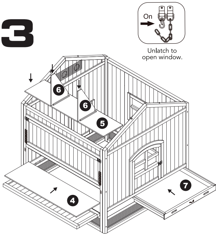
Insert Bottom Floor Board (4). Insert Nesting Box Board (5) and Divider Panels (6). Insert Cleaning Tray (7).
