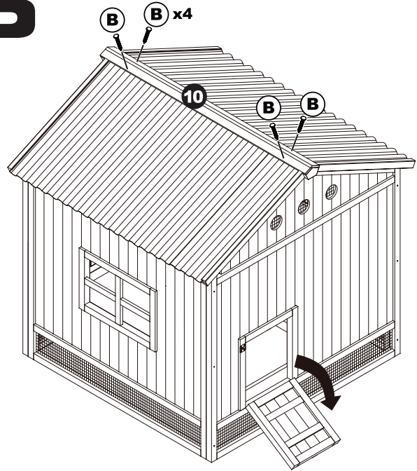
Attach Roof Cap (10) with Screws (B).
