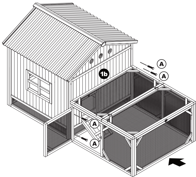
To connect KS-008 and KS-110 follow the arrow side with screws (A).
