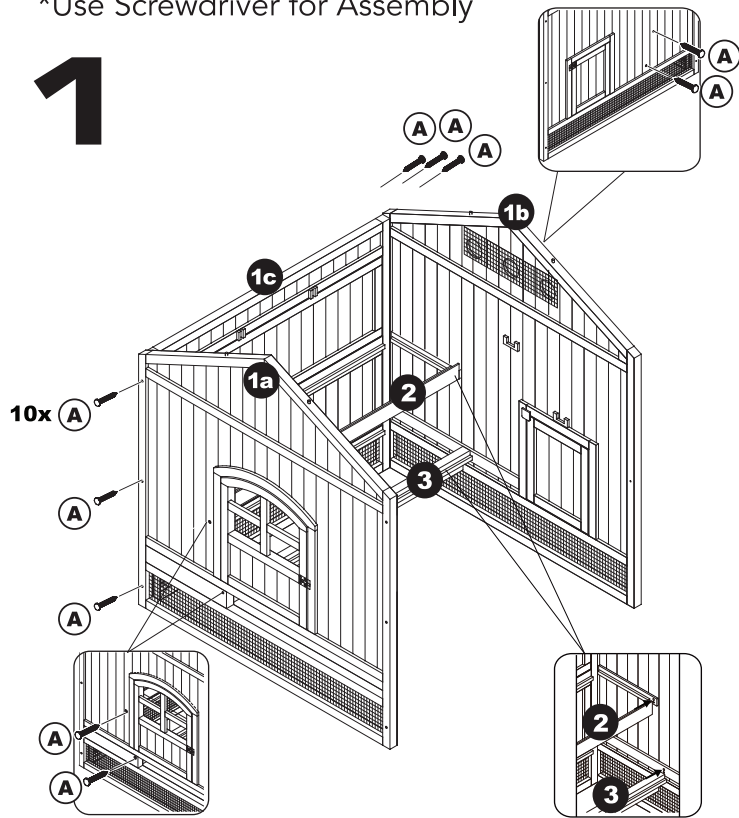
Connect Roosting Area Panels (1a, 1b, 1c) with Screws (A). Connect top connecting bar and bottom connecting bar (2, 3) with Screws (A).
