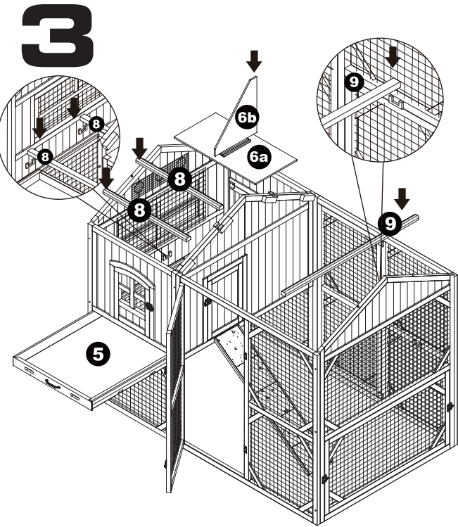
Insert Cleaning Tray (5). Insert Nesting Box Board (6a). Insert Nesting Box Divider (6b). Insert Internal Roosting Bars (8). Insert External Roosting Bar (9).
