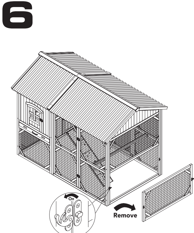
Front bottom panels can be removed by turning the lock.
