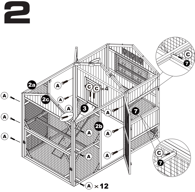
Connect Foraging Area Panels (2a, 2b, 2c) to Roosting Area with Screws (A). Attach Ramp (3) with Screws (C). Connect Floor Support Rail (7) with Screws (C).
