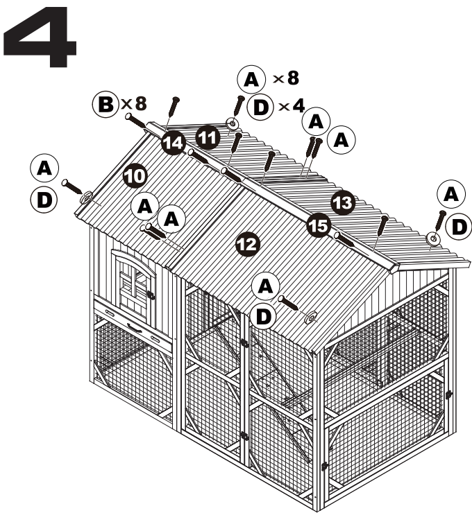
Attach Roosting Area Roof (10, 11) and Foraging Area Roof (12, 13) with Screws (A) and Plastic Washers (D). Attach Roosting Area Roof Cap (14) and Foraging Area Roof Cap (15) with Screws (B).
